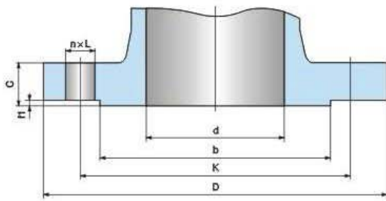
CLASS 150,300
