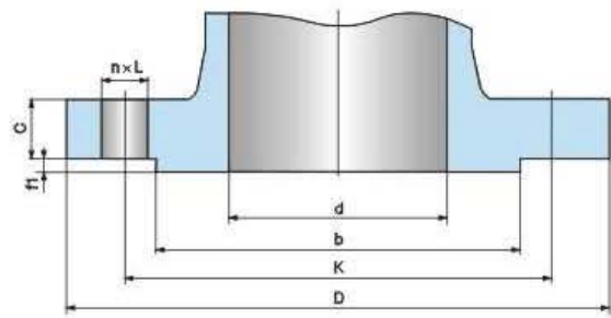
CLASS 600,900,1500,2500
